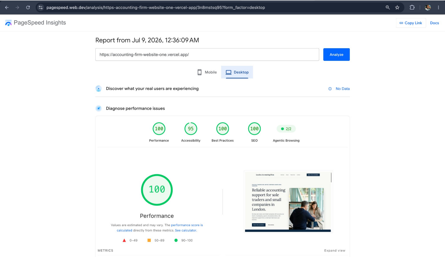
pagespeed-desktop-final.png
